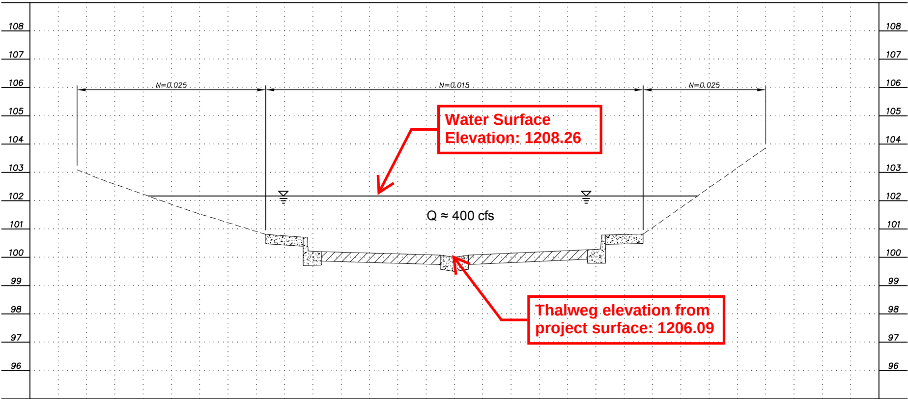
NORTH CROSS SECTION LOOKING DOWNSTREAM SCALE: H: 1"=10' V: 1"=3.33'
