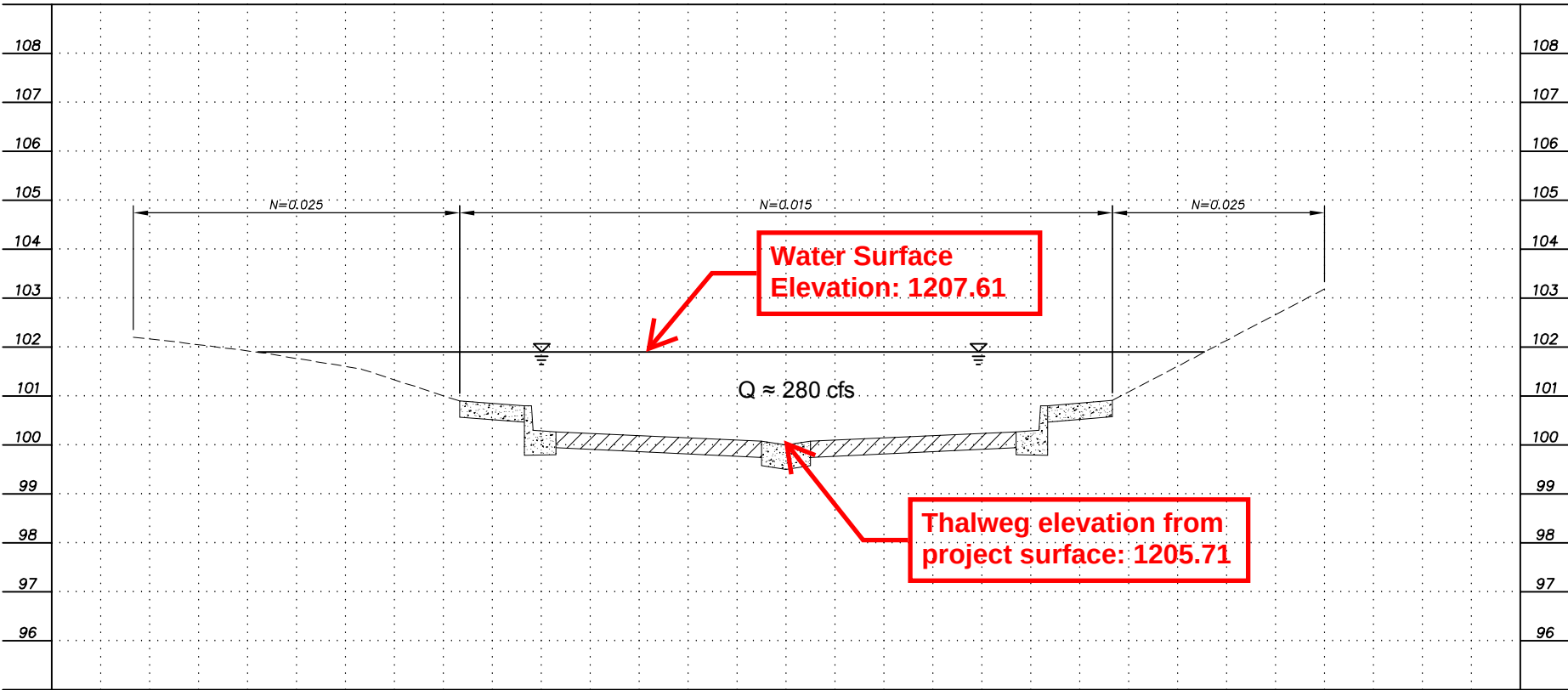
SOUTH CROSS SECTION LOOKING DOWNSTREAM SCALE: H: 1"=10' V: 1"=3.33'
